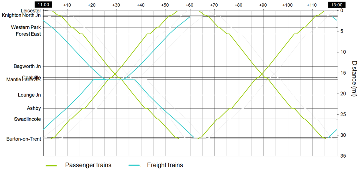
Figure 3.3: Train Graph Local Service (Rehabilitated Line Speeds)
