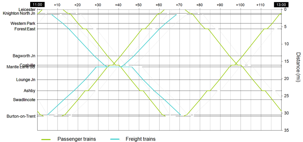
Figure 3.4: Train Graph Strategic Service(Rehabilitated Line Speeds)
