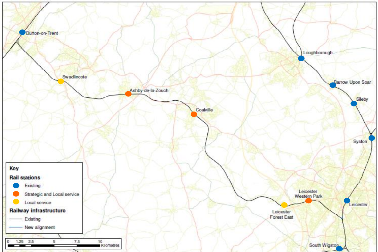
Figure 3.1: Leicester Burton Rail Alignment
