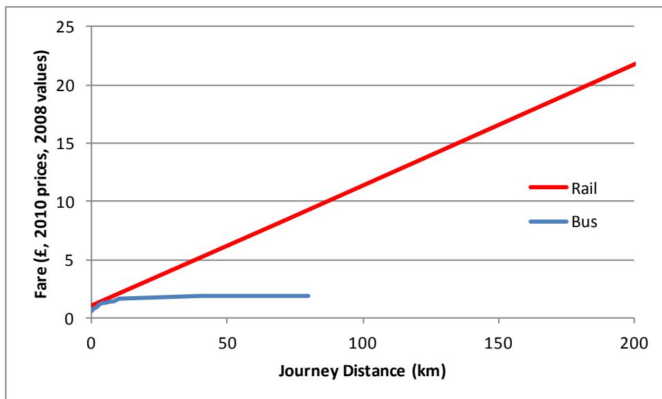
Figure 5.1: Fare Functions in LLITM
