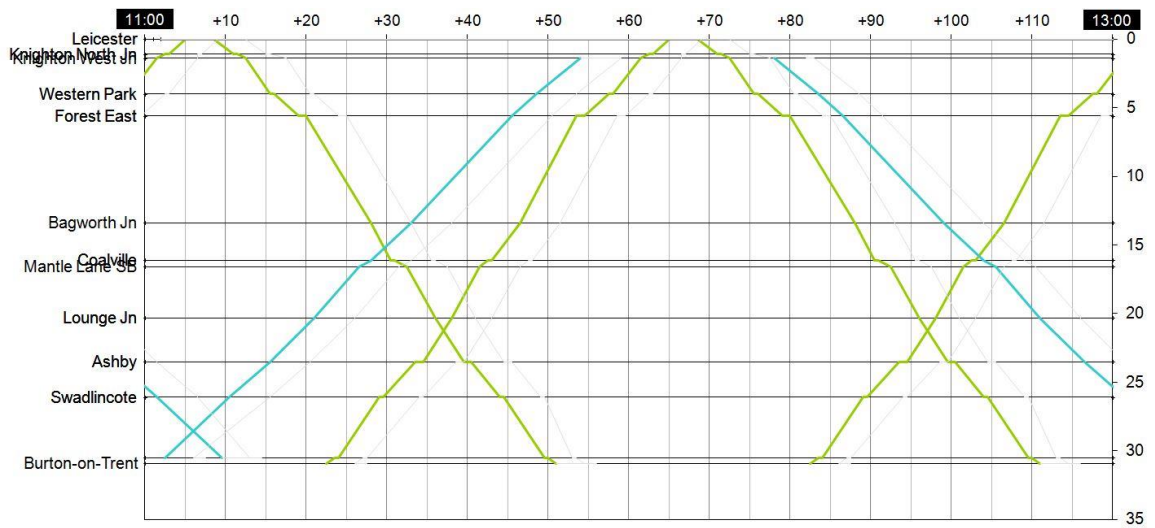
Figure 3.6: Train Graph Local Service- Maximum 75 mph
