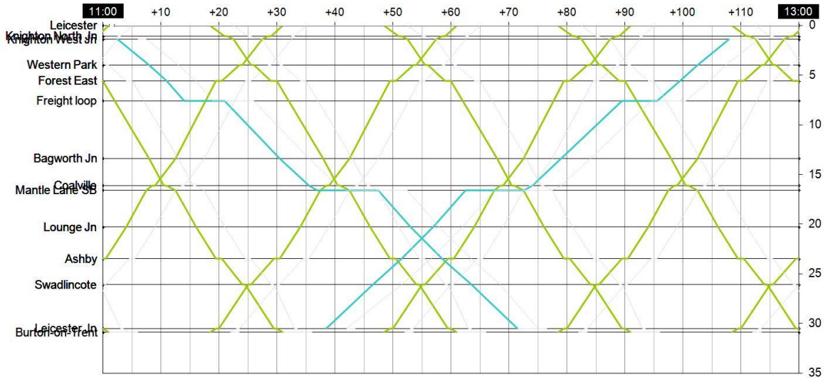
Figure 3.7: Train Graph Local Service- Maximum 75 mph and 2 Trains per Hour
