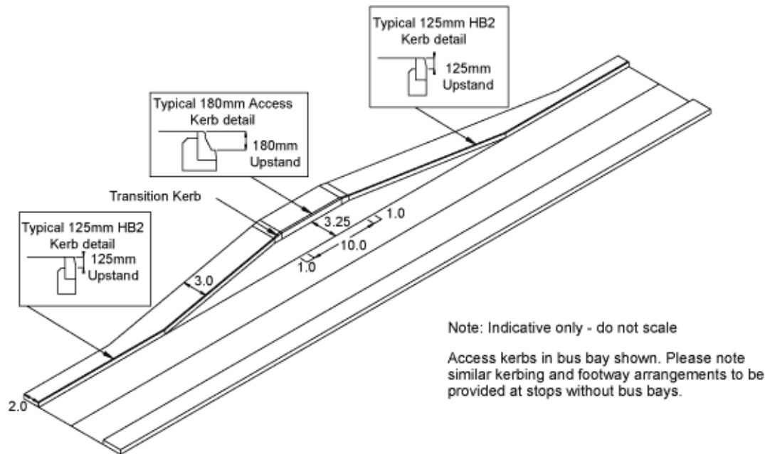
Figure DG8 Raised kerbing at bus stops
