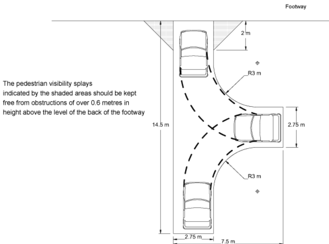
Figure DG22 Private drive turning facilities – typical example
