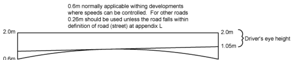
Figure DG2c Crests in road (brow of hill) Figure DG2 Construction of visibility splays
