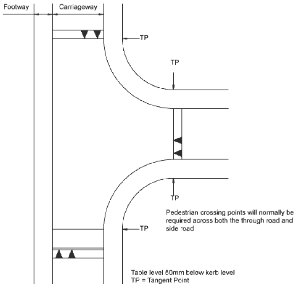
Figure DG6d Junction table (please also see Part 4, paragraph 4.86)
