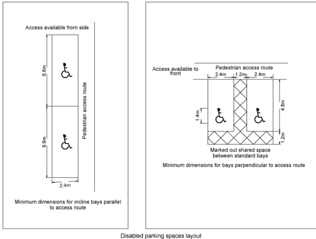
Figure DG16 Size and layout of parking spaces. Minimum parking space 2.4m x 5.5m
