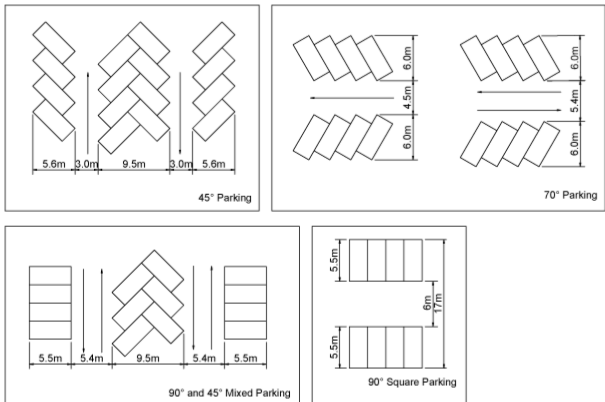
Example parking layouts
