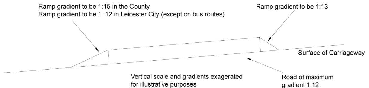
Figure DG6e Cross section of speed tables with alterations for steep roads shown in lower diagram (please also see Part 4, paragraph 4.86)
